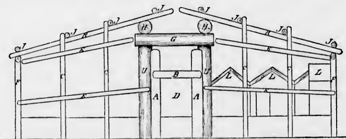
FIG. 3. Construction of Kwakiutl house. Front elevation.
